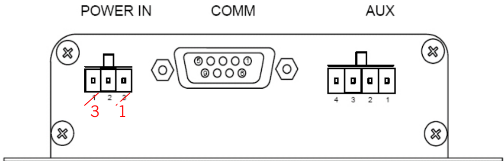
Figure 4.4: Connector Pinouts
